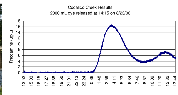
Characterizing pollutant transport using dye releases (photo and graph showing data results).
